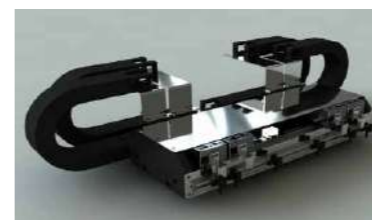
Multi-Mover Stage
