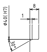
A部詳細図 Enlarged detail A
